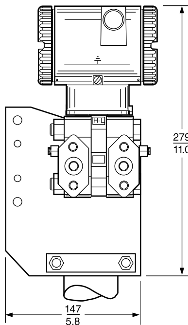
VERTICAL PIPE MOUNTING
