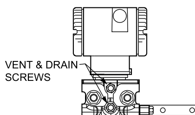
Figure 15 - Low Profile (LP2) Transmitter – Shown on a Coplanar Bracket
