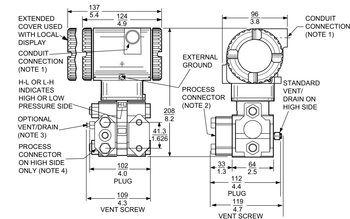
Figure 27 - Biplanar AP/GP Transmitters
