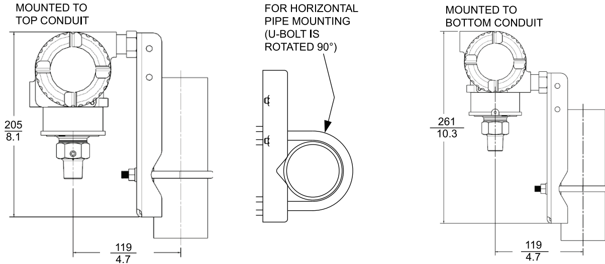
Figure 24 - Direct Connect AP/GP Transmitters with Options -M1, -M2, -M5, and -M6
