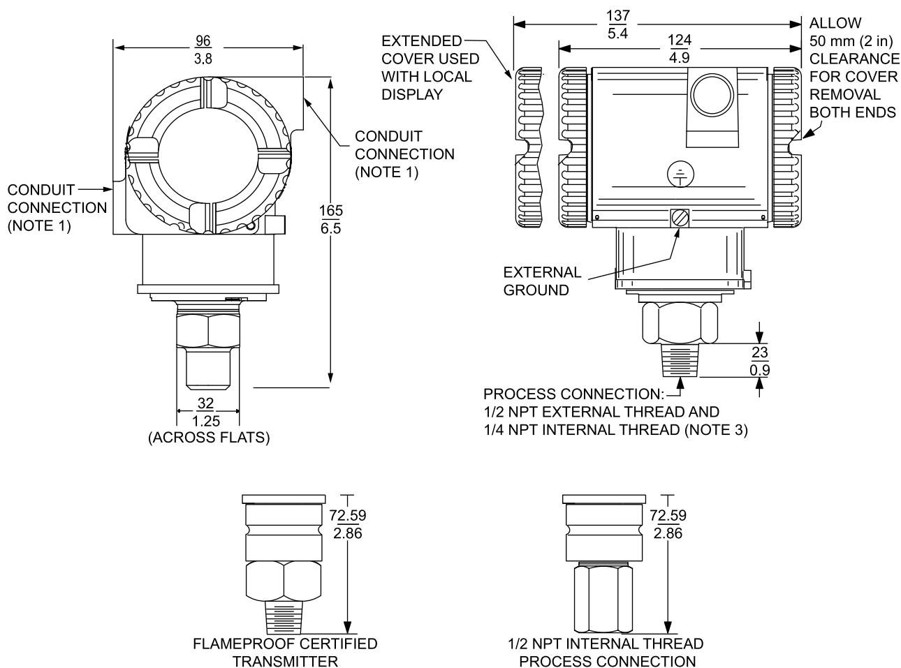
Figure 22 - Direct Connect AP/GP Transmitters
