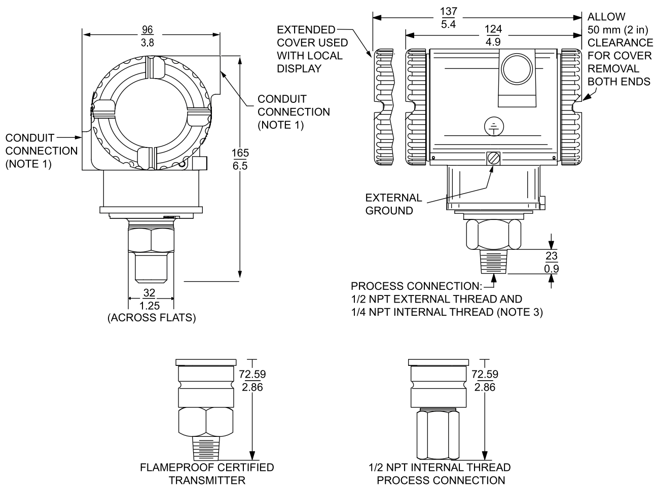
Figure 23 - Direct Connect AP/GP Transmitters
