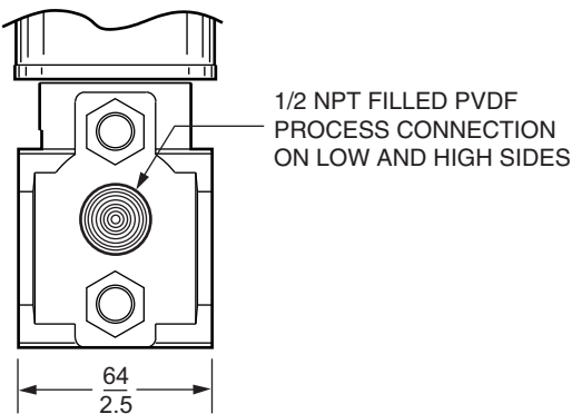
Figure 37 - DP Transmitters with Traditional Structure and Structure Codes -78 and -79 (Filled PVDF Connection)
