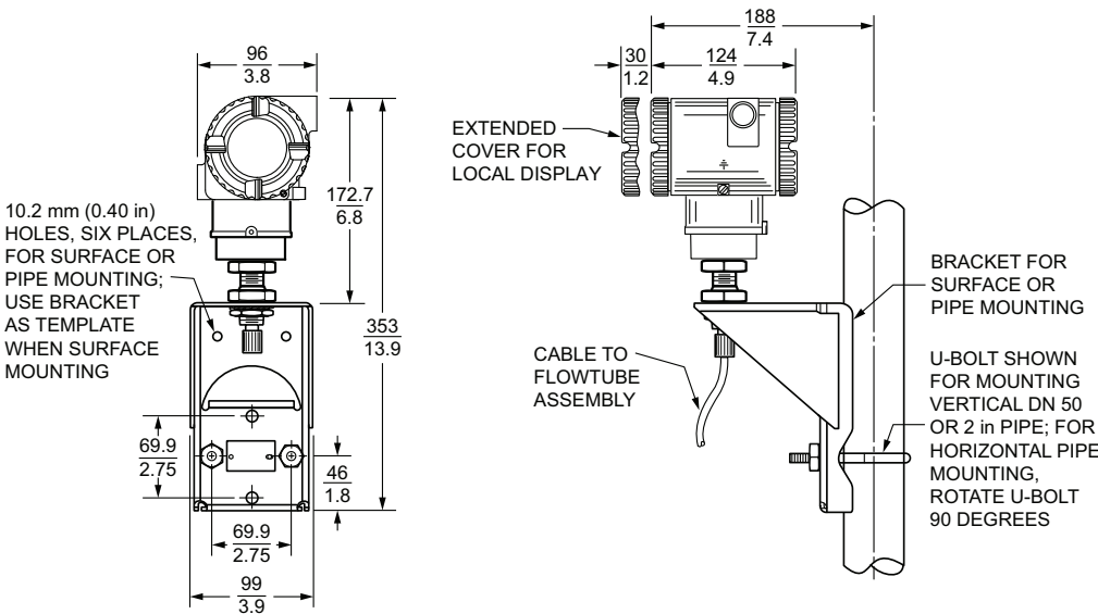
Figure 12 - Remotely Mounted Electronics Housing for 84CS
