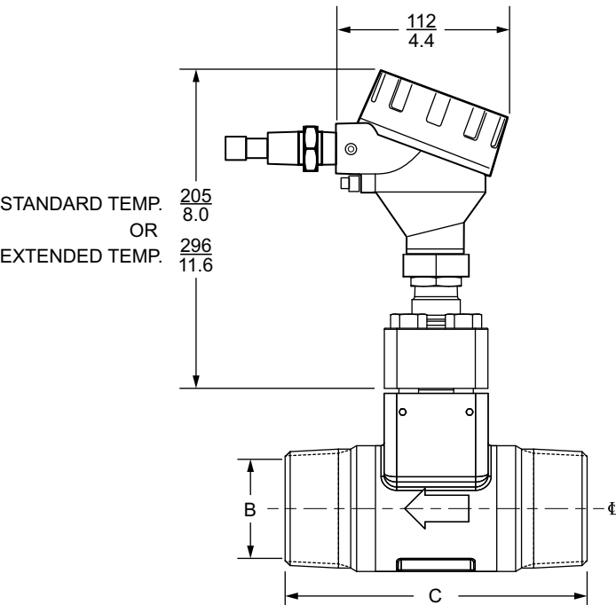
Figure 10 - NPT Body Flowmeter with Junction Box
