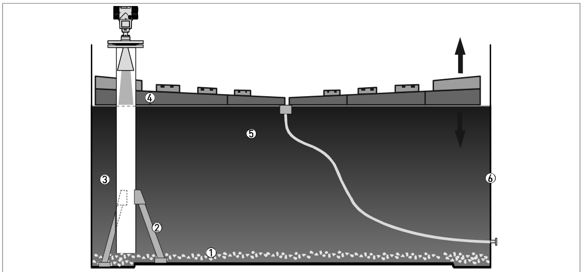
Figure 3-17: Floating roofs
