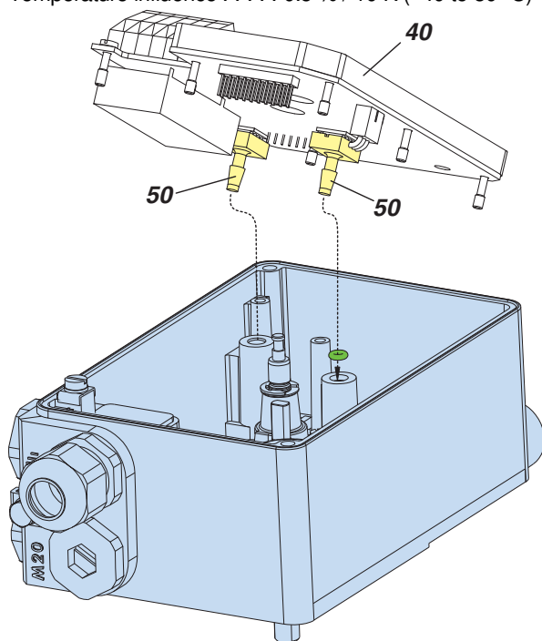
Pressure sensors 50
